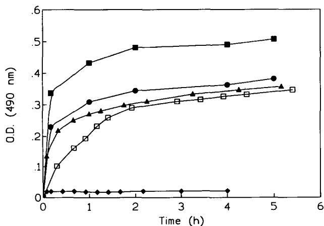
Figure 3. Turbidimetric analysis (micro-quantitative precipitation) of Con A ( 1 \text{ mg mL}^{-1} ) with yeast mannan at 0.5 \text{ mg mL}^{-1} (▲) and 16-mer manno-dendrimer 18 at 0.5 \text{ mg mL}^{-1} (■) and at 0.25 \text{ mg mL}^{-1} (●). Inhibition effect of p -nitrophenyl \alpha -D-mannopyranoside on binding of Con A to yeast mannan (◆). The measurements were done in PBS using an ELISA plate reader at 25^\circ\text{C} .
