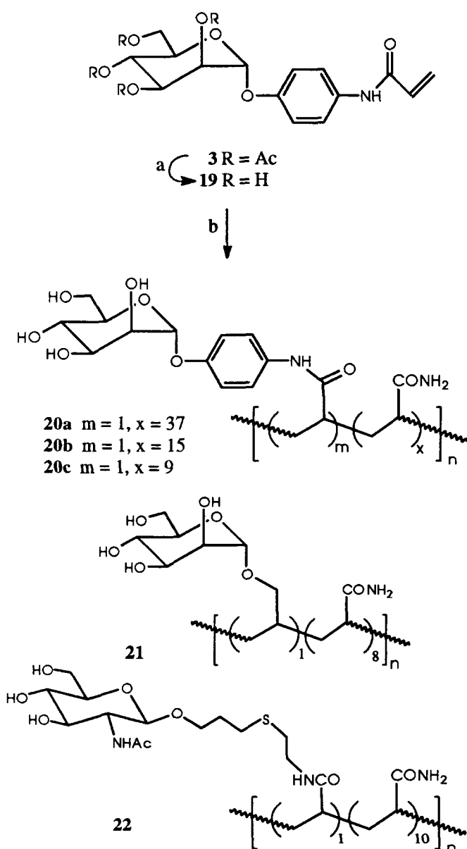
Scheme 3. Reagents and Conditions: (a) NaOMe, MeOH, 2 h, r.t., 99%; (b) CH 2 =CH-CONH 2 , (NH 4 ) 2 S 2 O 8 , H 2 O, N 2 , 25 min, 90 °C, 67%.
