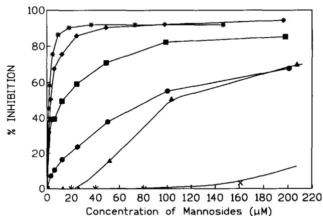
Figure 4. Inhibition of binding of Con A to yeast mannan by Man- \alpha -OMe (X), Man- \alpha -OPh- p -NO 2 (▲), and mannosylated dendrimers 12 (●), 14 (■), 16 (◆), and 18 (*).
