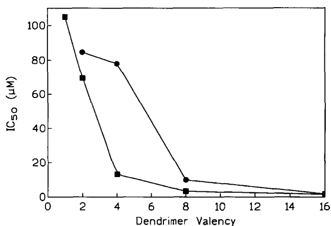
Figure 5. Effect of dendrimer valency on the inhibition of binding of Con A to yeast mannan (■) and pea lectin to mannose-co-polymer 20a (●).
