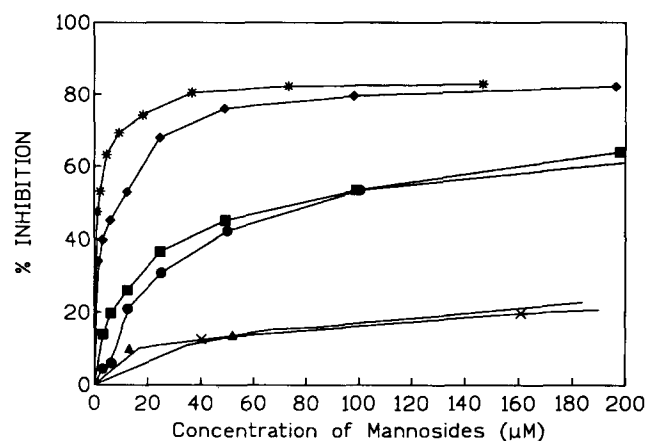
Figure 6. Inhibition of binding of pea lectin to mannose-co-polymer 20a by Man-α-OMe (X), Man-α-OPh- p -NO 2 (▲), and mannosylated dendrimers 12 (●), 14 (■), 16 (◆), and 18 (*).
