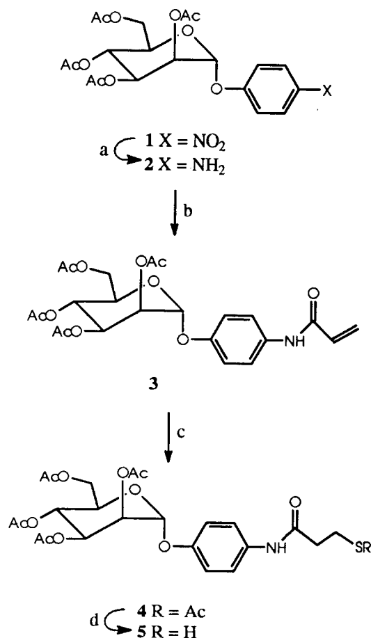
Scheme 1. Reagents and conditions: (a) 10% Pd-C, \text{NH}_4\text{HCO}_3 , MeOH, 30 min, 94%; (b) \text{CH}_2=\text{CH}-\text{COCl} , \text{Et}_3\text{N} , \text{CH}_2\text{Cl}_2 , 0 \rightarrow 25 ^\circ\text{C} , 45 min, 75%; (c) AcSH, \text{K}_2\text{CO}_3 , \text{CH}_3\text{CN} , 5 h, r.t., 81%; (d) \text{H}_2\text{NNH}_2\text{-HOAc} , DMF, \text{N}_2 , 20 min, 25 ^\circ\text{C} , 92%.
