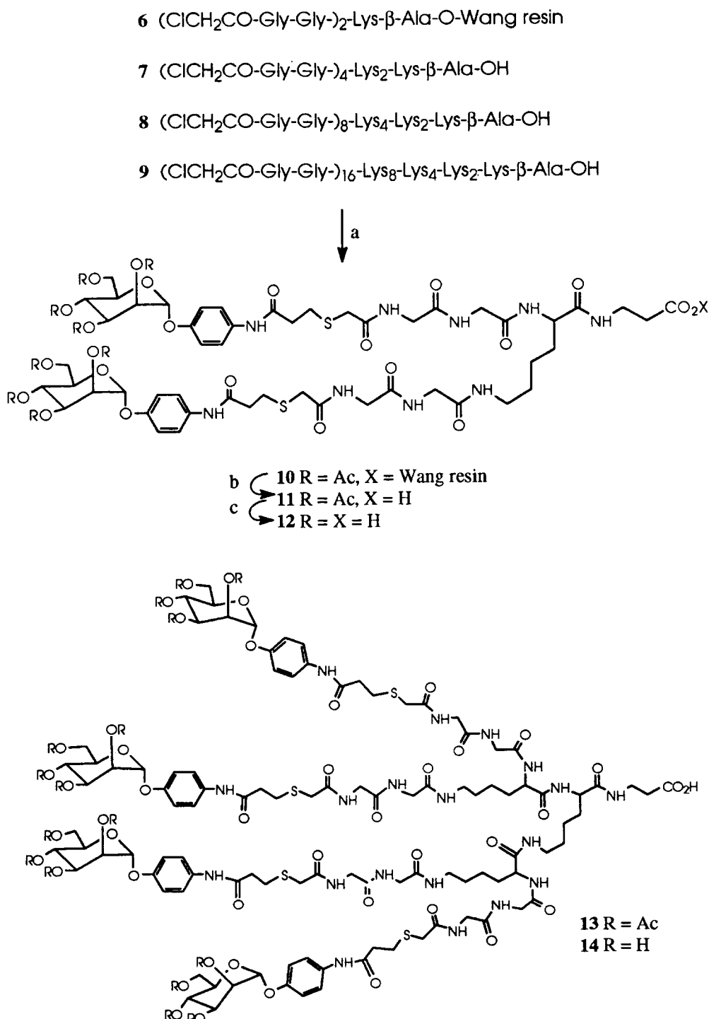
Scheme 2. Reagents and conditions: (a) thio-mannoside 5 , 1% DIPEA, DMF; (b) 95% aq TFA, 25 °C, 1.5 h; (c) NaOMe, MeOH.
