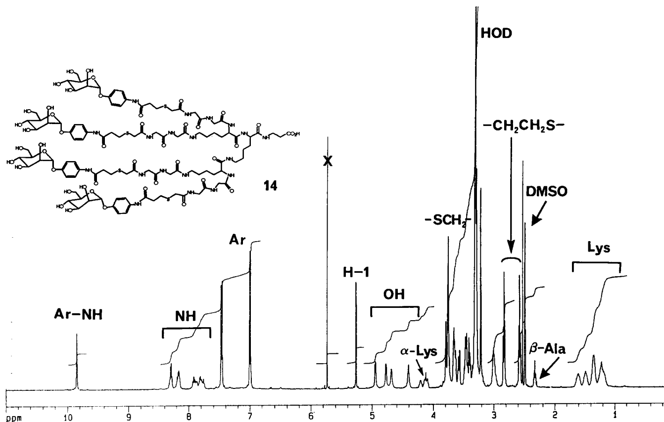
Figure 1. 500 MHz ^1\text{H} NMR spectrum ( \text{DMSO}-d_6 ) of tetraivalent mannosylated dendrimer 14 .
