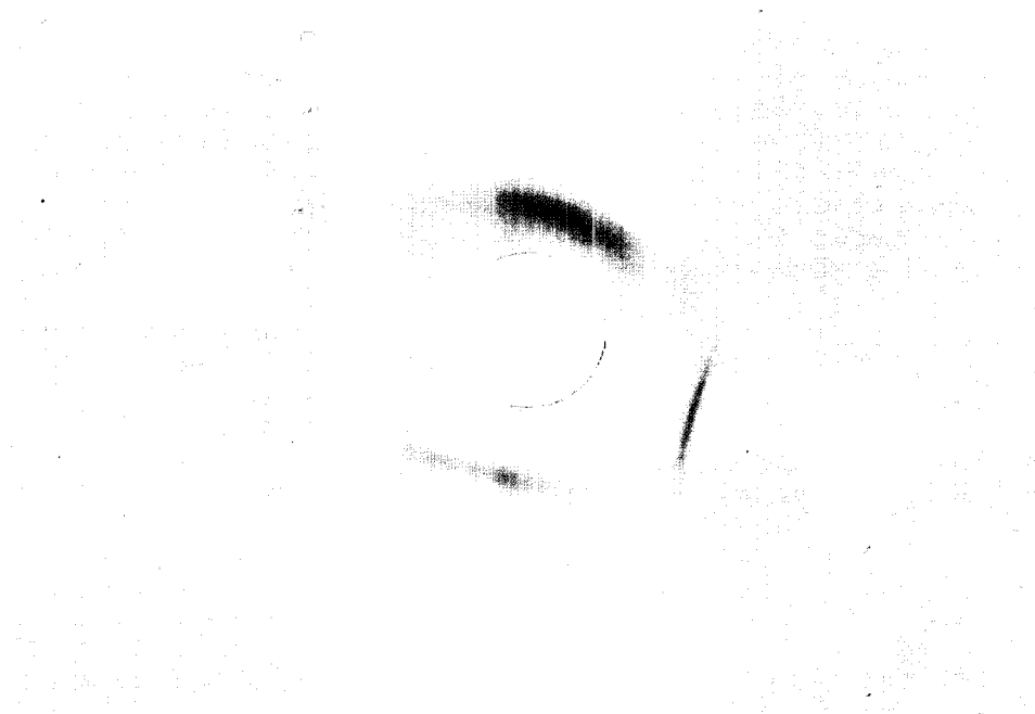
Figure 2. Agar gel diffusion of Con A (middle well) against poly(acrylamide-co-allyl \alpha -D-mannopyranoside) ( 21 ), positive control (bottom well); poly(acrylamide-co- \beta -D-N-acetylglucosaminide) ( 22 ), negative control (left well); 16-mer mannosylated dendrimer 18 (top well); poly(acrylamide-co-4-acrylamidophenyl \alpha -D-mannopyranoside) 20c (right well).
